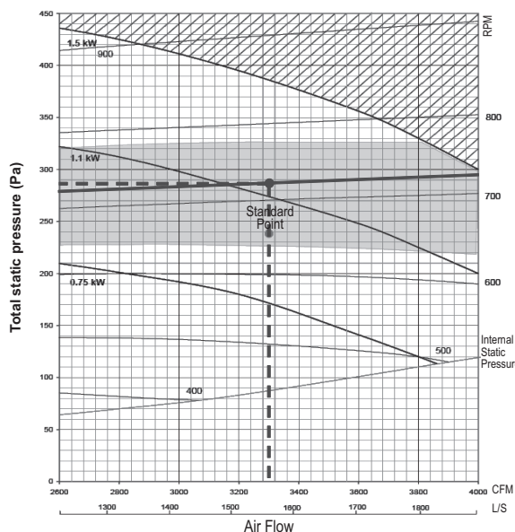
UATYQ250 - blower curve
